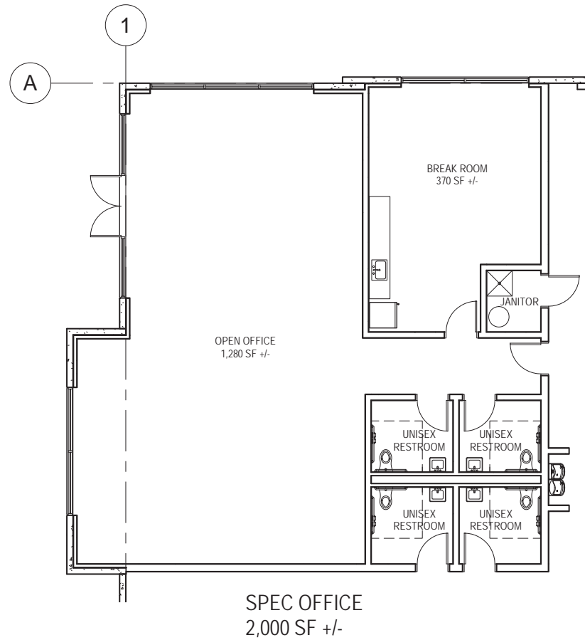
1 SPEC OFFICE - FLOOR PLAN 1/8" = 1'-0"
